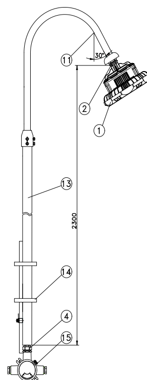
Flange Stanchion
